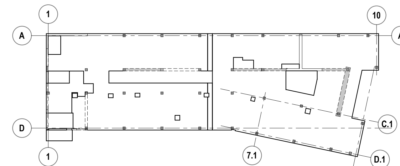
KEYPLAN LEVEL 03
