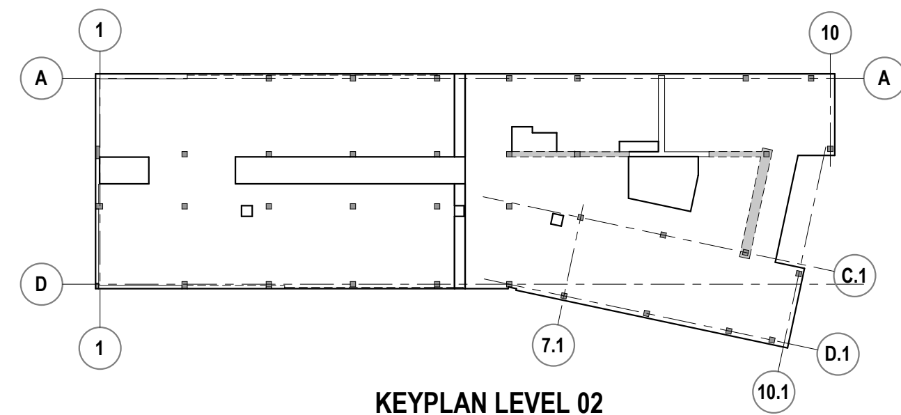
KEYPLAN LEVEL 02
