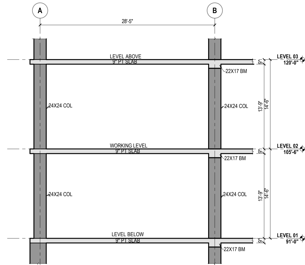
2 BUILDING ELEVATION - LEVEL 02
