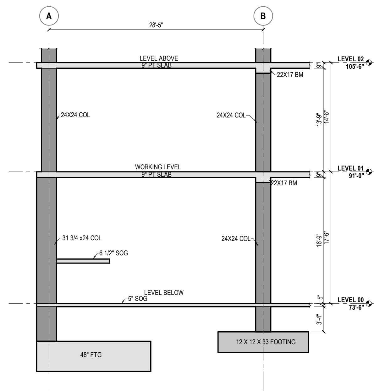
2 BUILDING ELEVATION - LEVEL 01 1/8" = 1'-0"
