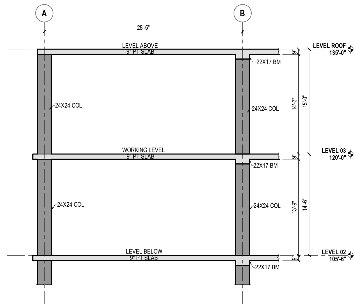
2 BUILDING ELEVATION - LEVEL 03
