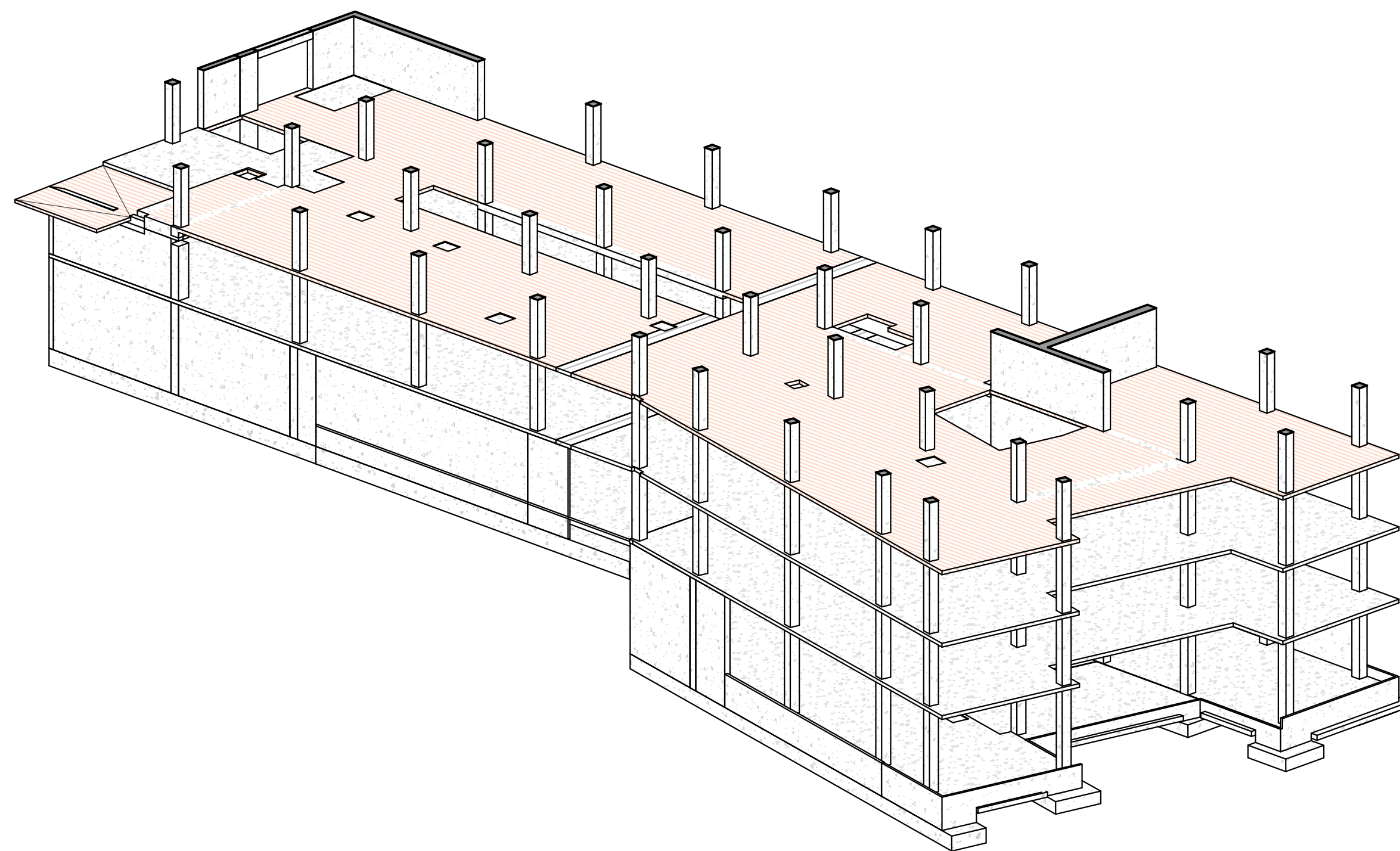
3 3D VIEW - LEVEL 03
